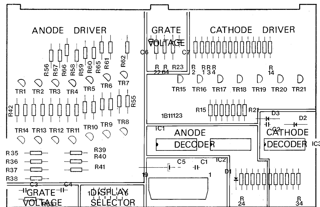
C.P.U. BOARD
