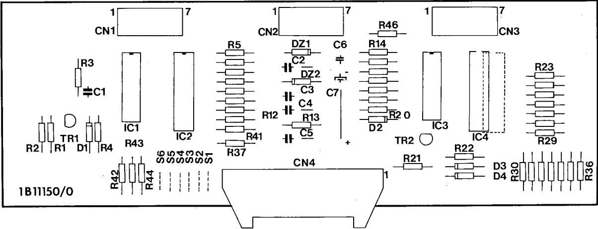
EB 0256 8 DIGIT DISPLAY DRIVER BOARD (1B1150/0) ASS.
