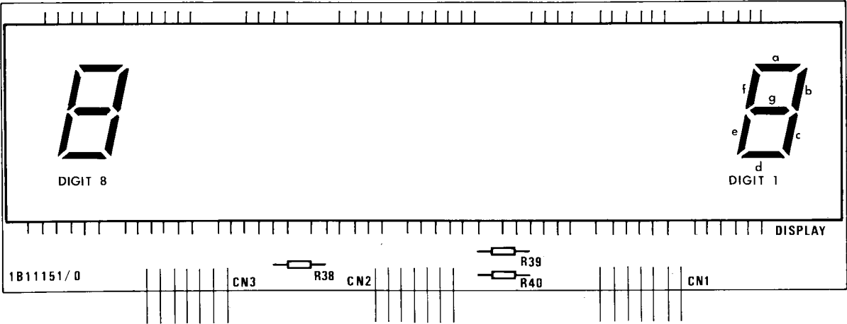
EB 0257 8 DIGIT DISPLAY BASE BOARD (1B1151/0) ASS.
