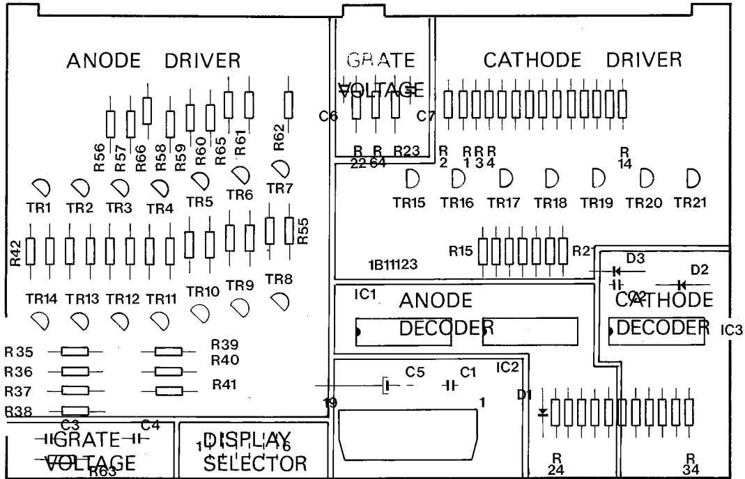
C.P.U. BOARD
